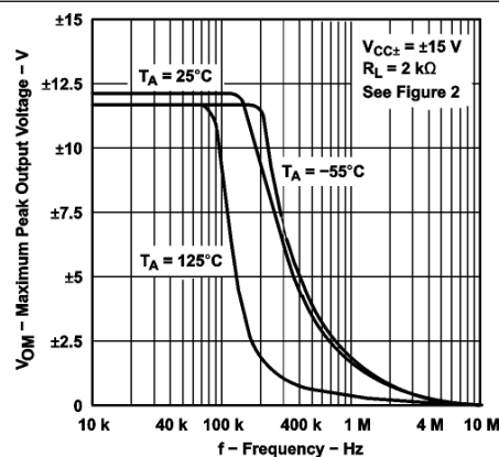
Figure 5-39. Maximum Peak Output Voltage vs Frequency
